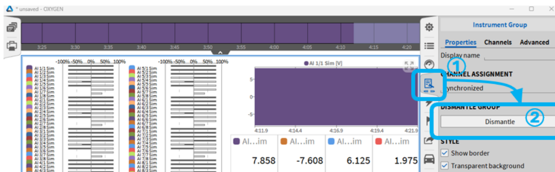
Fig. 8.6: 拆分乐器组
