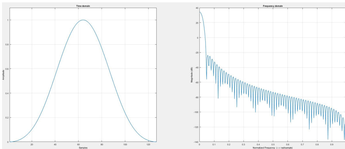
Fig. 8.60: Blackman 窗时域和频域特征图 (N = 128)
