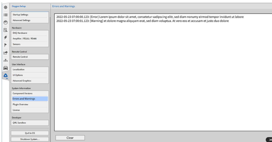
Fig. 6.29: 错误和警报
