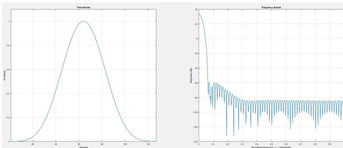
Fig. 8.61: Blackman-Harris 窗时域和频域特征图 (N = 128)
