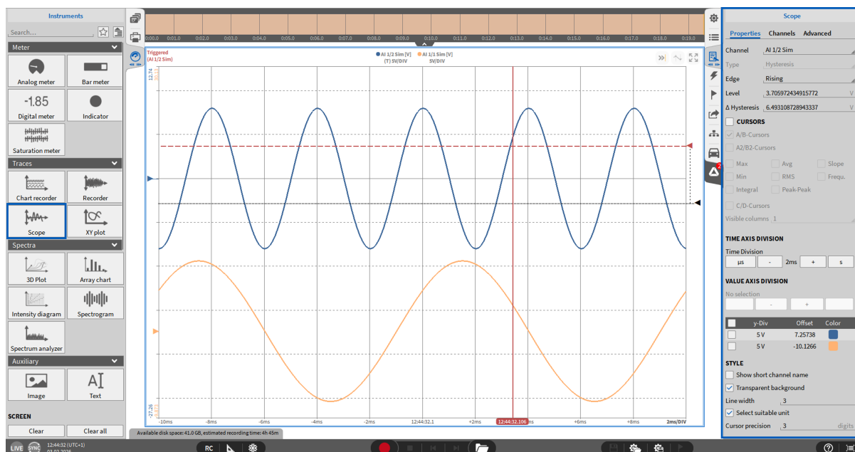
Fig. 8.38: 示波器-总览
