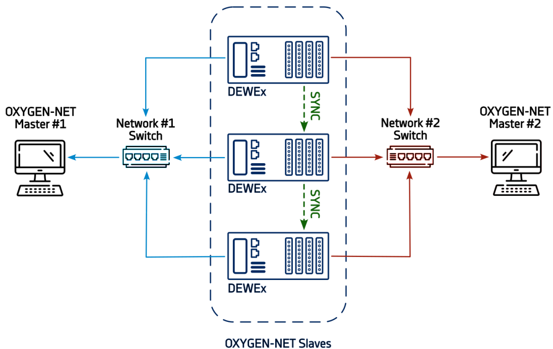
Fig. 15.4: Multi-Master system based on two different networks
