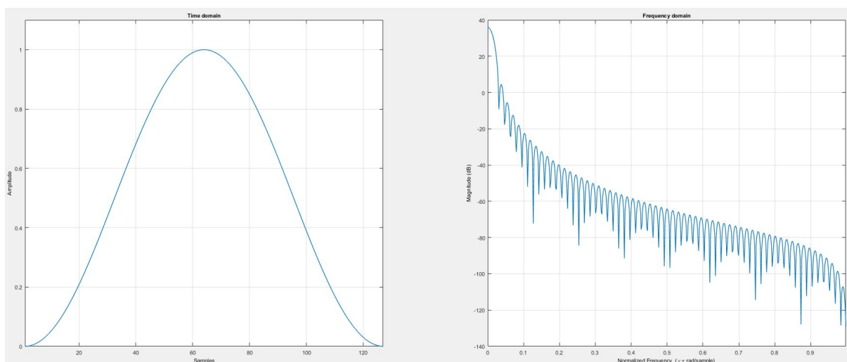
Fig. 8.57: Hanning window in time and frequency domain (N = 128)
