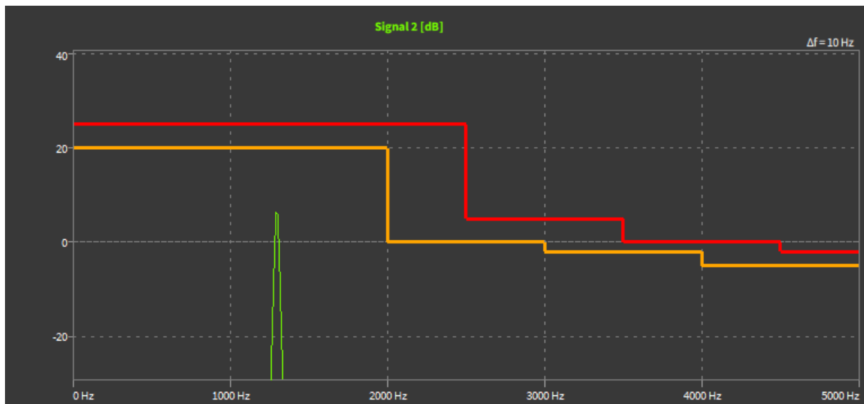
Fig. 8.72: Reference curves without limit exceeded
