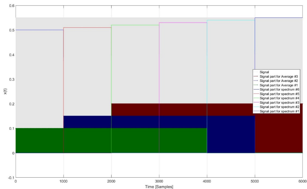
Fig. 8.96: Decomposition of the time signal for a Periodogram with an average of 4 spectra and 0 % overlapping
