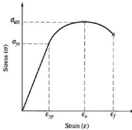
Fig. 7.117: Strain-Stress-Curve
