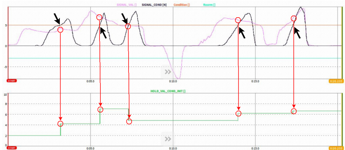
Fig. 7.61: HOLD function with Condition and Initial value
