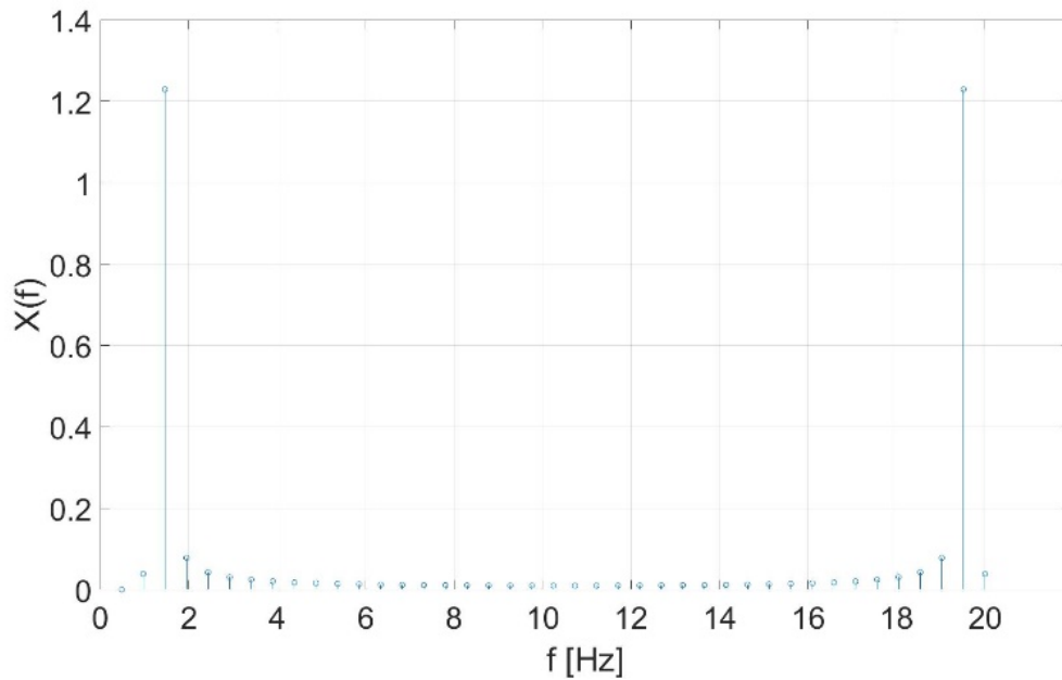
Fig. 8.79: Signal 1 in frequency domain, no zero-padding
