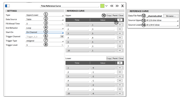
Fig. 7.119: Properties of the time reference curve
