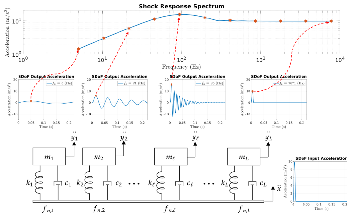
Fig. 7.150: Schematic procedure for calculating a shock response spectrum
