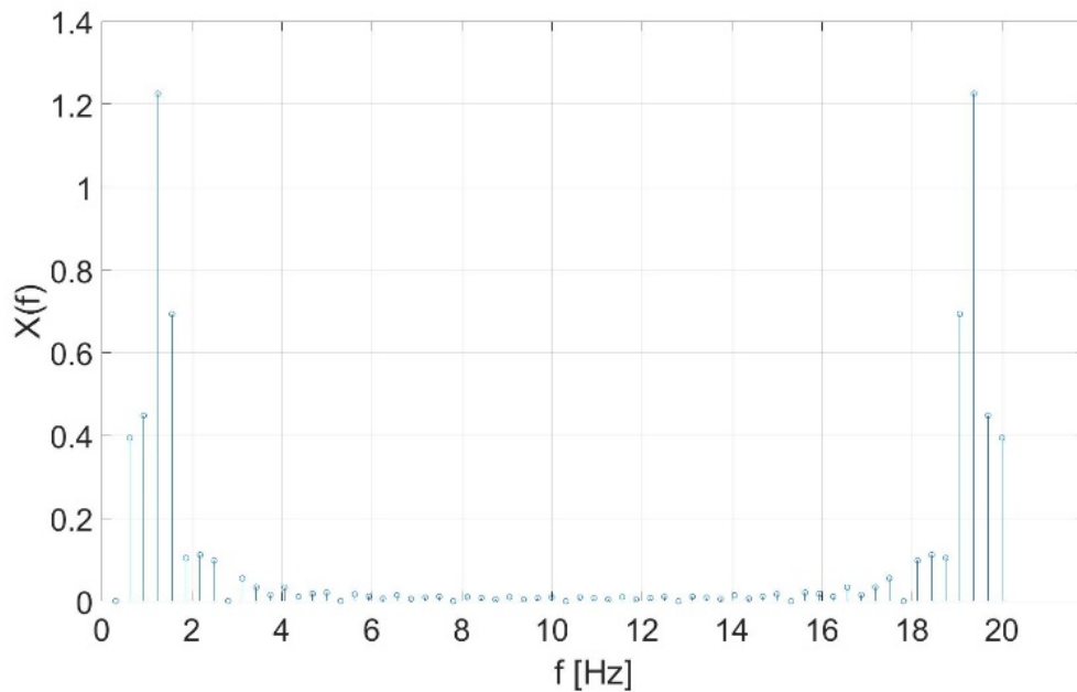
Fig. 8.81: Signal 1 in frequency domain, zero-padding to 64 samples
