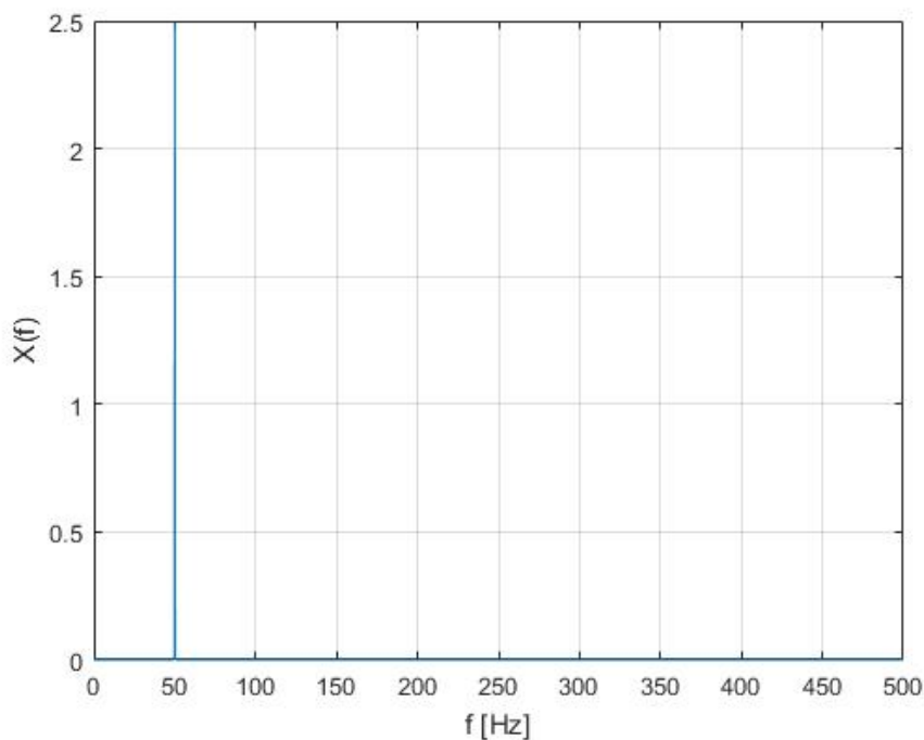
Fig. 8.94: Amplitude-True-normalized spectrum X(f)
