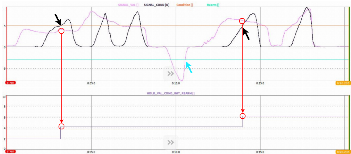
Fig. 7.62: HOLD function with Condition , Initial value and Rearm level
