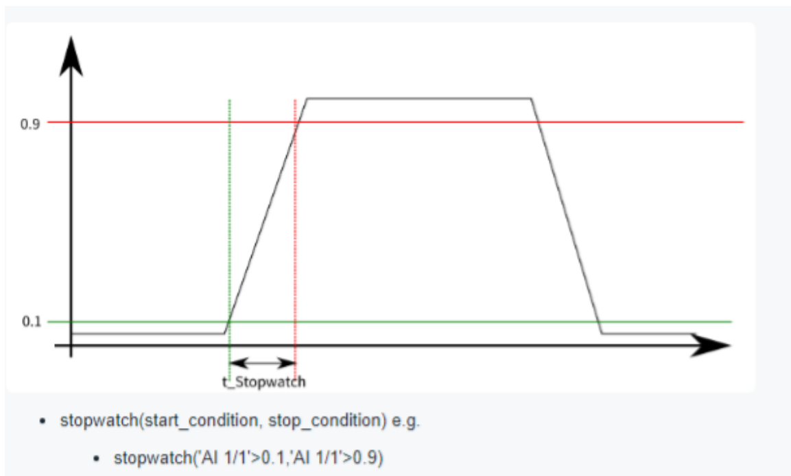
Fig. 7.63: Schematic explanation of the stopwatch function
