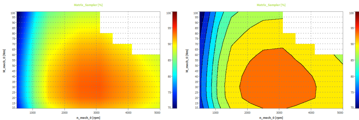
Fig. 8.50: Intensity Diagram of a Matrix Sampler channel without (left) and with level grading (right, 10 levels)
