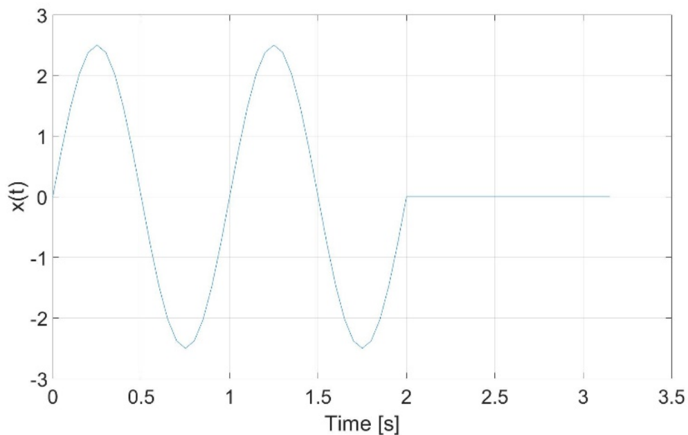
Fig. 8.80: Signal 1 in time domain, zero-padding to 64 samples
