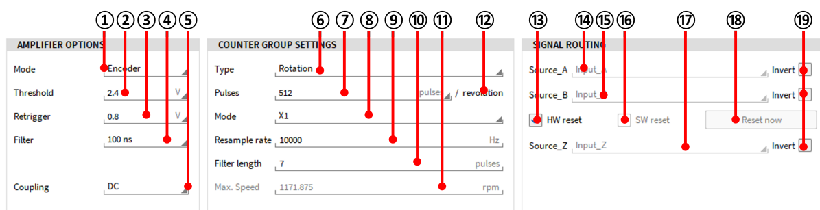
Fig. 7.195: Channel Setup for a TRION-CNT channel in Encoder mode
