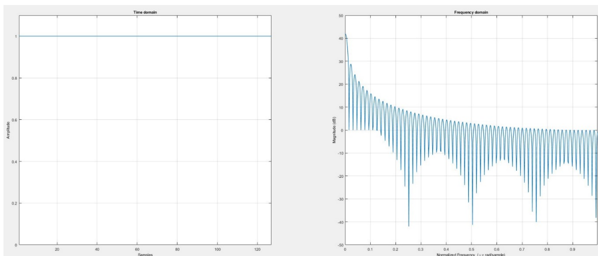
Fig. 8.59: Rectangular window in time and frequency domain (N = 128)
