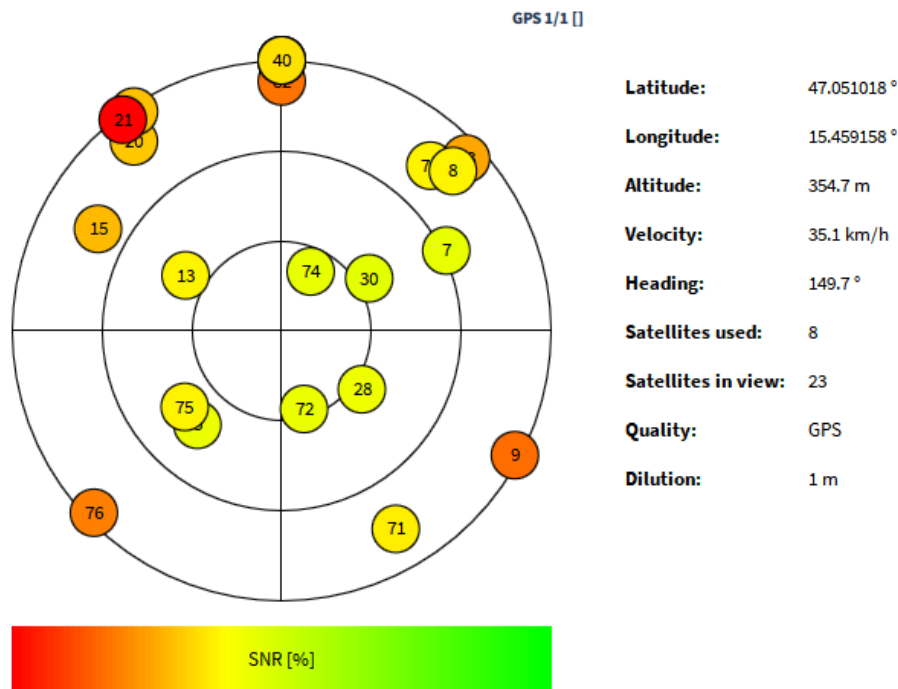
Fig. 8.106: GPS Quality instrument - overview
