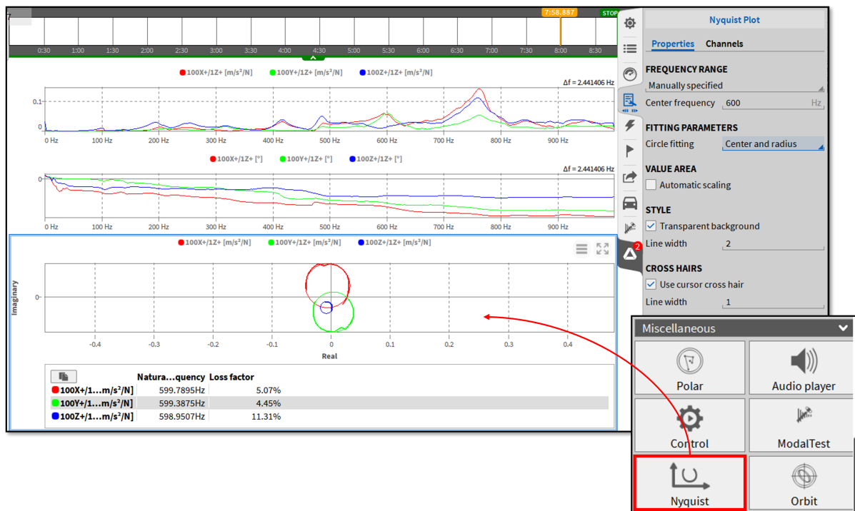
Fig. 8.121: Nyquist Plot properties
