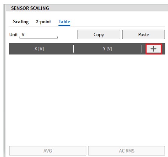
Fig. 7.41: Table scaling – add point to specify x- and y-value
