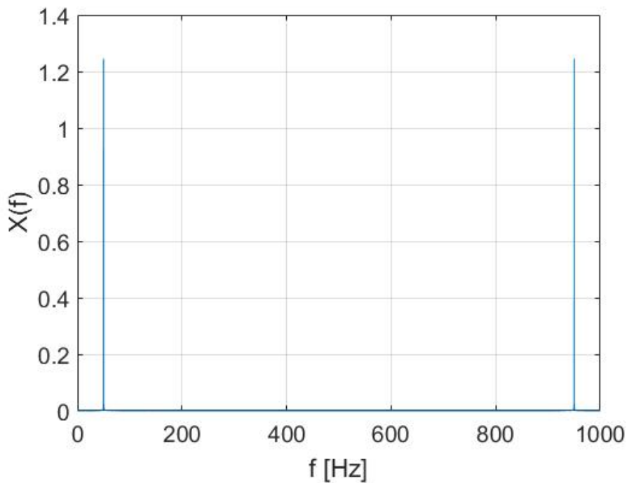
Fig. 8.88: x(t) in frequency domain divided by the FFT-length
