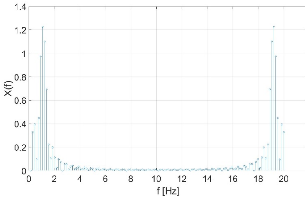
Fig. 8.83: Signal 1 in frequency domain, zero-padding to 128 samples
