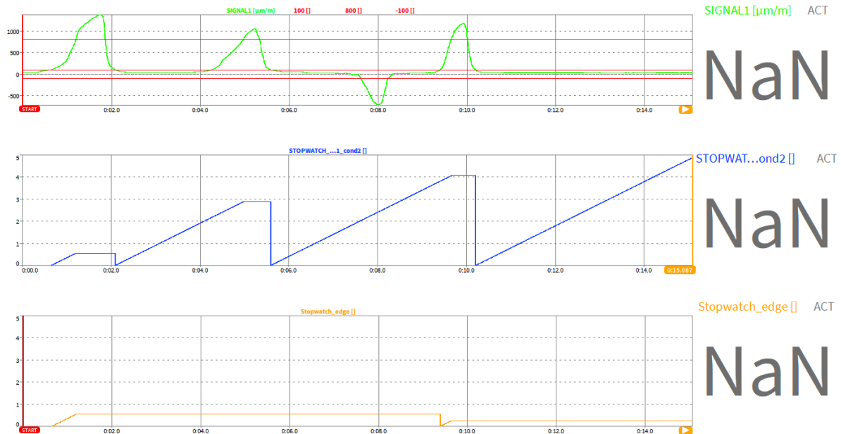
Fig. 7.73: Combination of edge and stopwatch function
