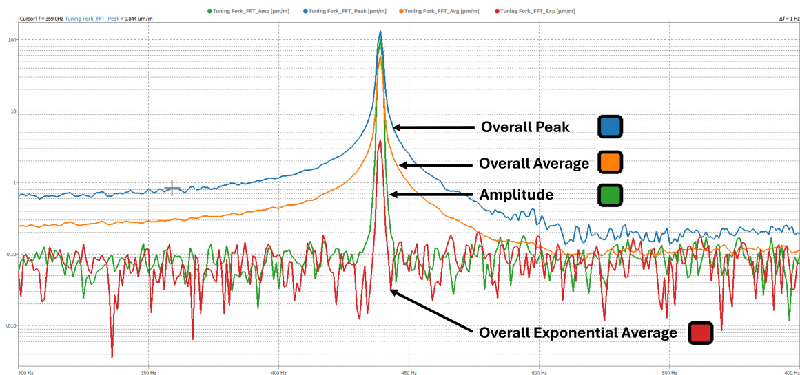
Fig. 7.93: Example of amplitudes, overall peak, overall RMS average, overall exponential average in the spectral view
