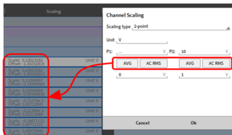
Abb. 7.24: AVG & ACRMS calibration for multiple channels
