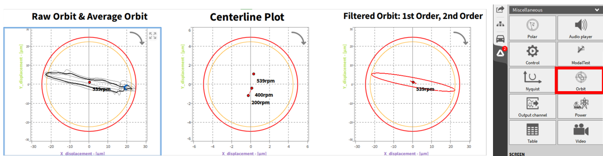
Abb. 8.122: Orbit Plot Instrument
