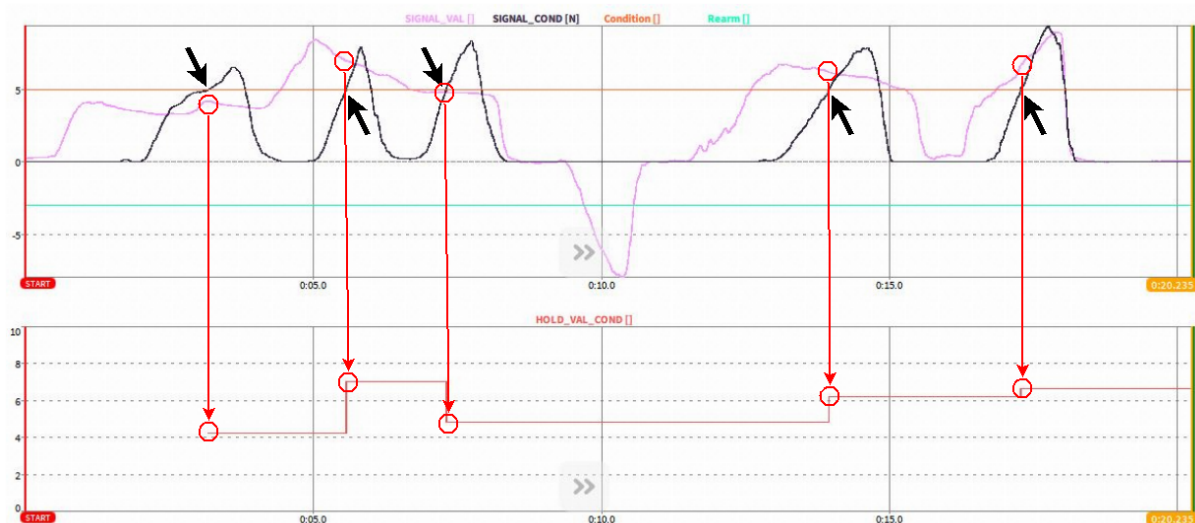
Abb. 7.60: HOLD function with Condition
