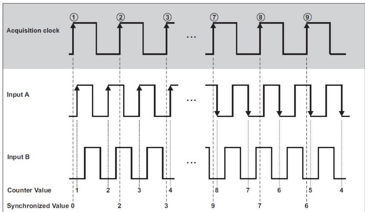
Abb. 7.187: Quadrature Encoder X1 Mode
