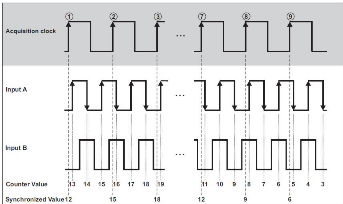
Abb. 7.188: Quadrature Encoder X2 Mode
