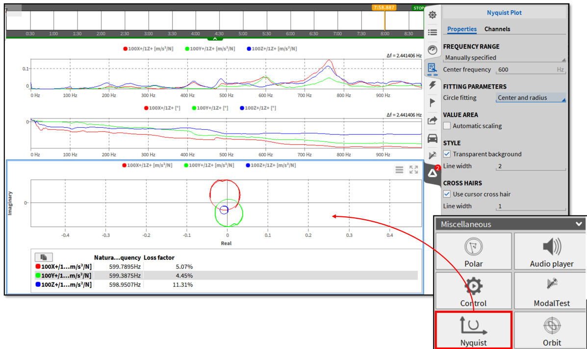
Abb. 8.121: Nyquist Plot Eigenschaften
