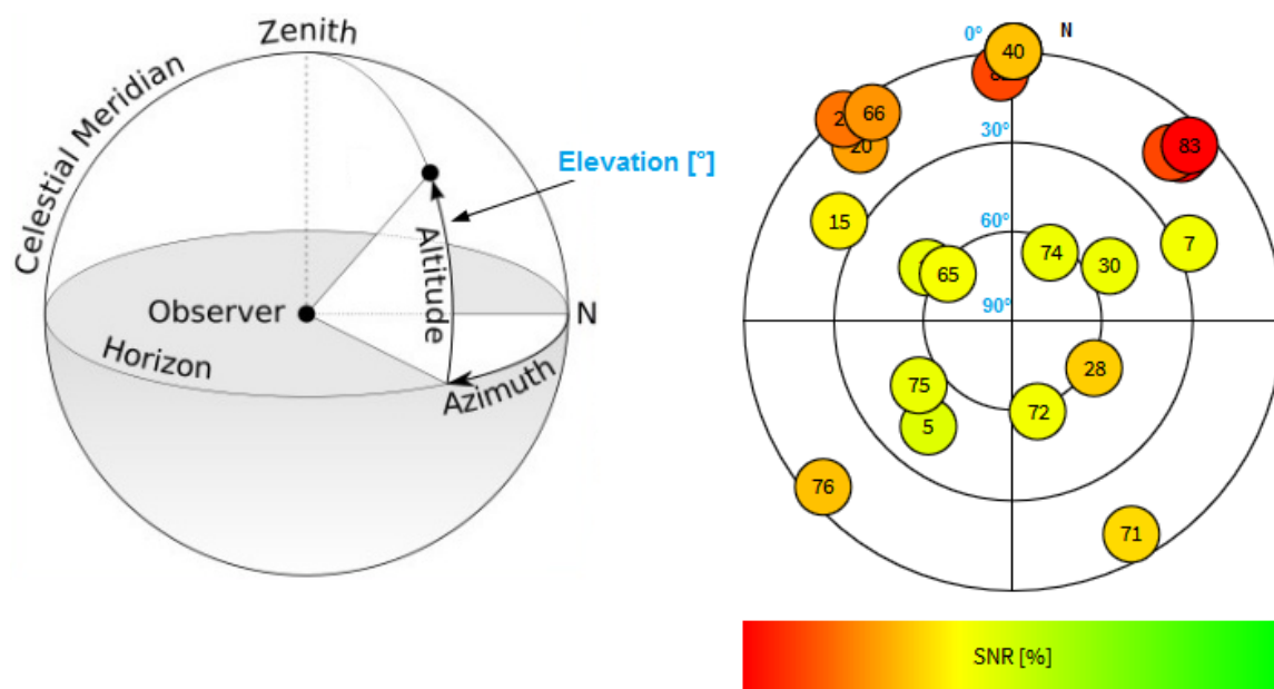
Abb. 8.108: Explanation of the satellites plot
