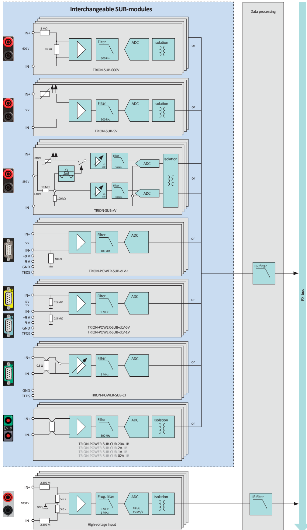
Fig. 156: Block diagram
